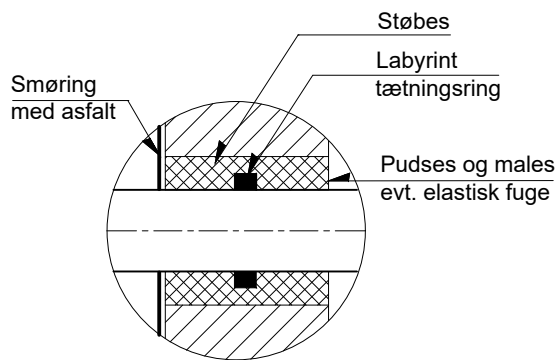
Detailje 1
