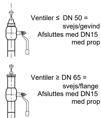
Detailje 1
